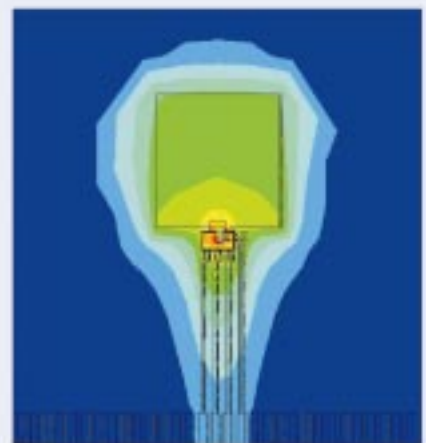
SOT223-4-2 on a PCB with 6 cm² heat sink; R_{thj-a} \sim 70 \text{ K/W} is calculated at P_V = 0.5 \text{ W}
